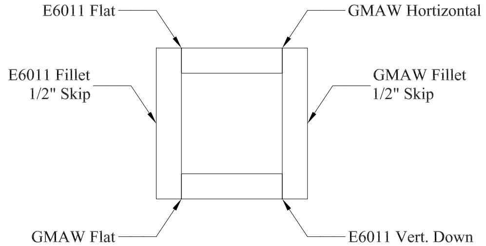
Weld Location Detail
