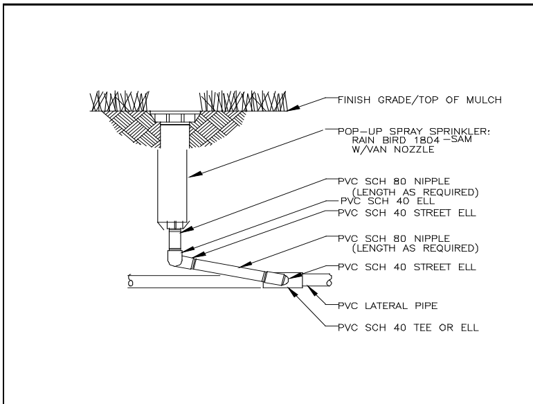
Figure 8 – Pop-up Spray Sprinkler
