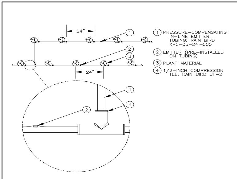
Figure 10 – Xeri-Tube_PC
