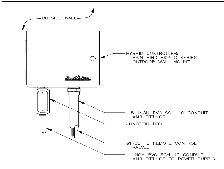
Figure 5 – Hybrid Controller
