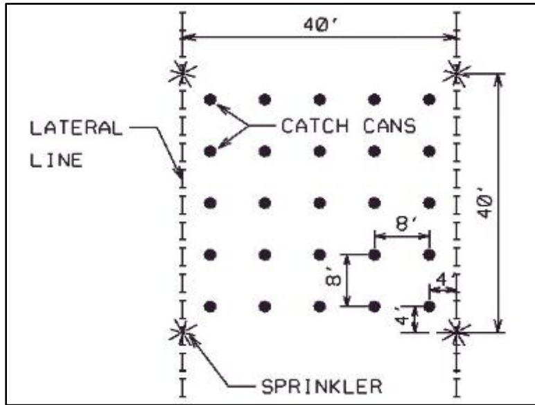
Figure 4a – Example Solid Set Catch Can Layout
