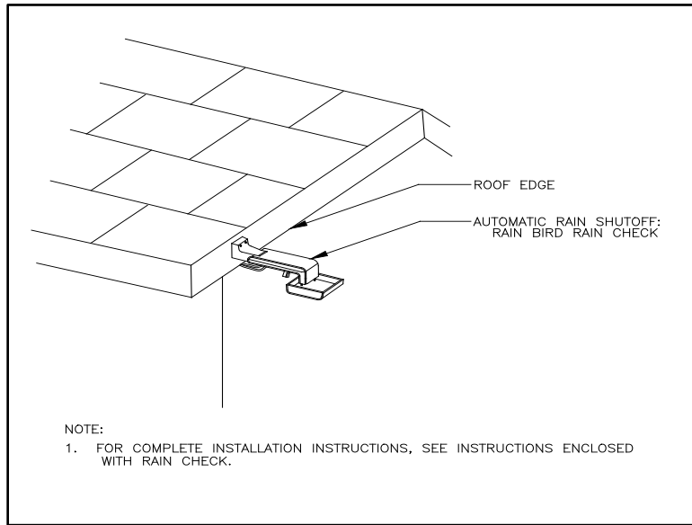
Figure 11 – Automatic Rain Shutoff
