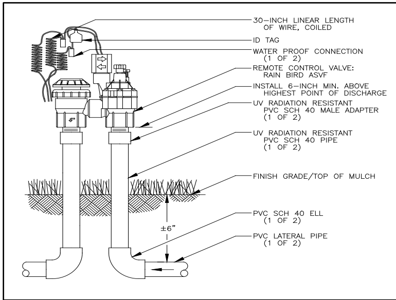
Figure 7 – Remote Control Valve
