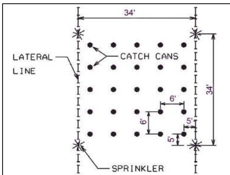
Figure 4b – Example Solid Set Catch Can Layout
