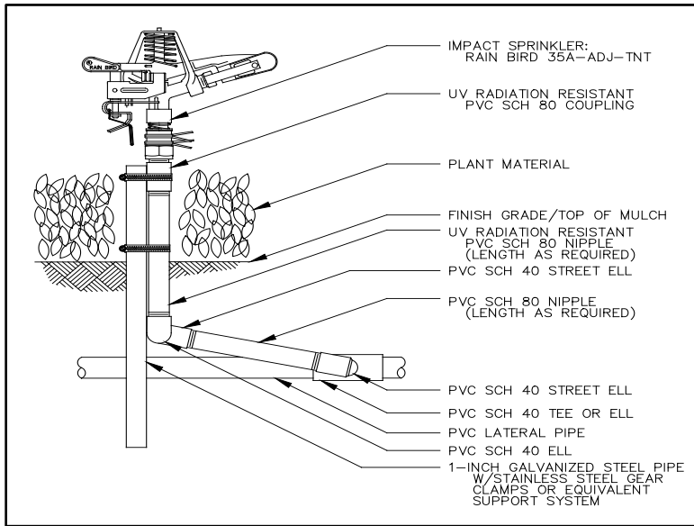
Figure 9 – Impact Sprinkler
