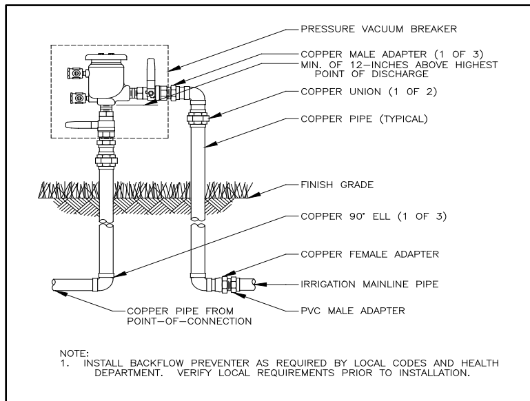
Figure 6 – Pressure Vacuum Breaker
